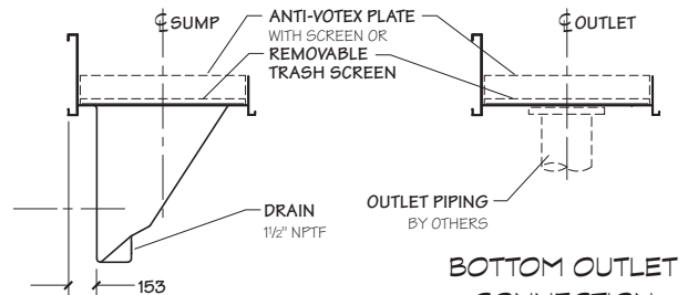
SUMP SECTION
