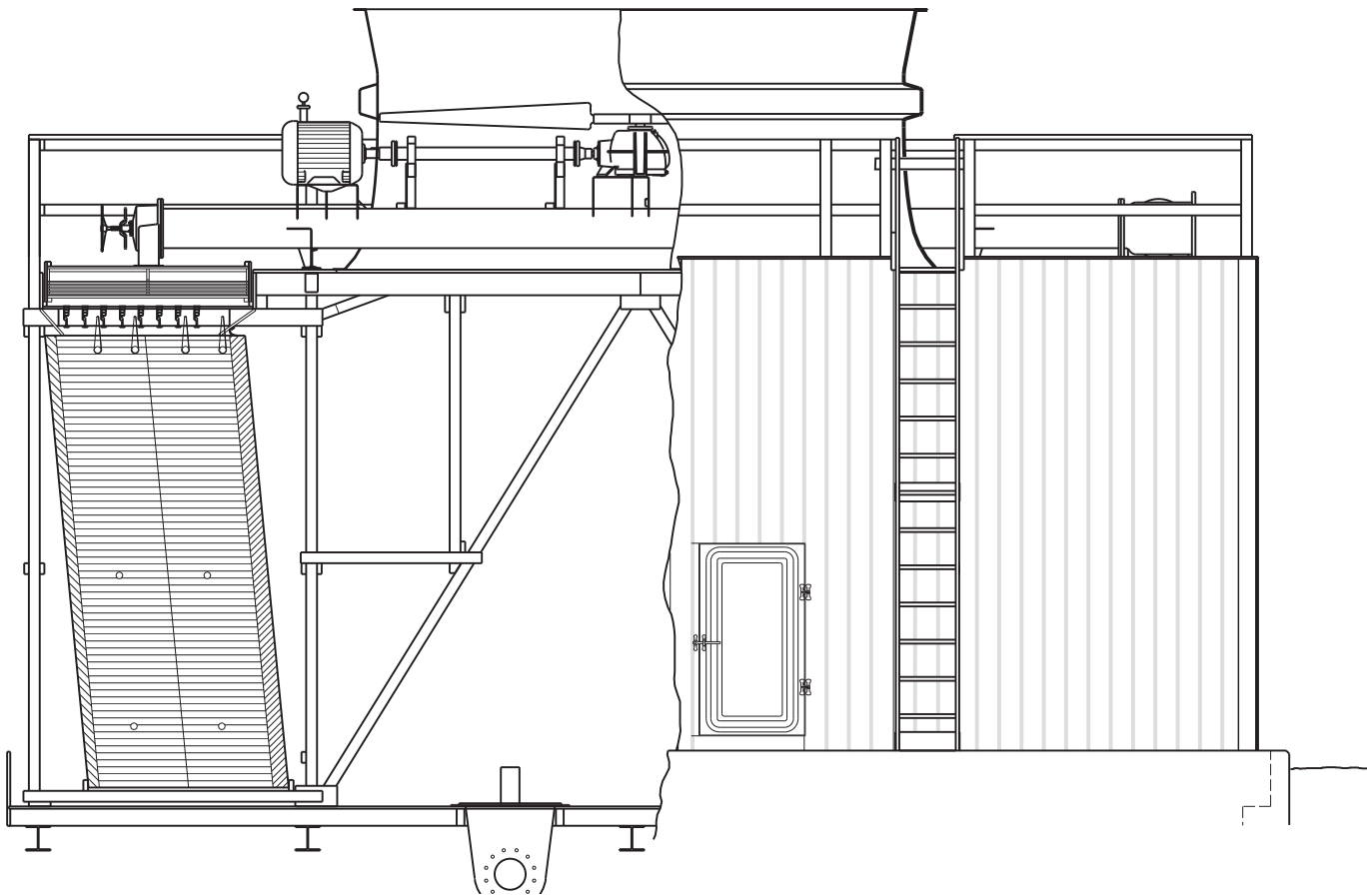
Series 1200 Cross-Section
