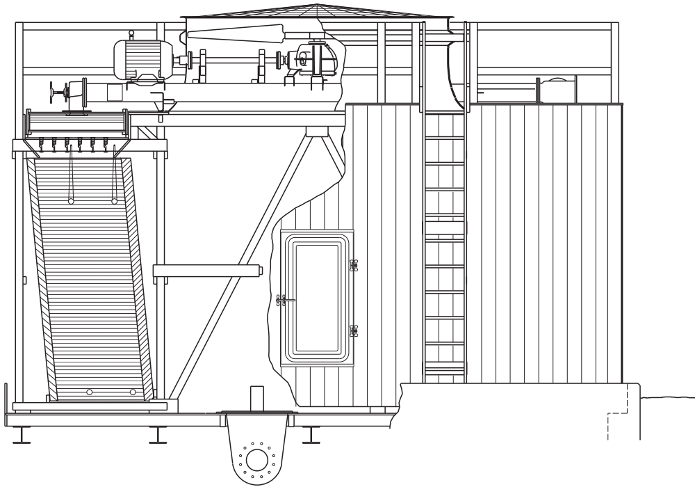
Series 1000 Cross-Section
